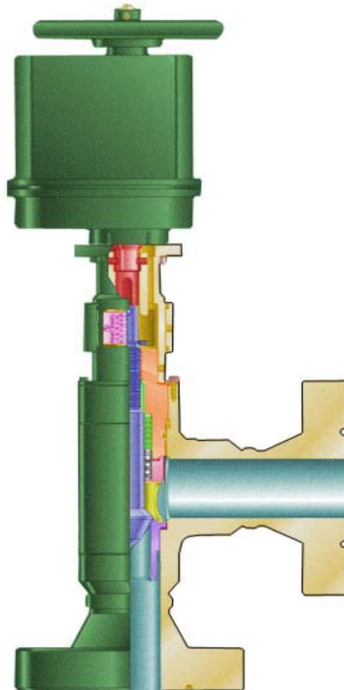
ACV Valve with Electric Actuator
