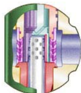
Cavrosion-Cavnoise Valve Trim
