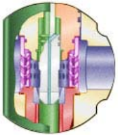
Cavnoise Valve Trim
